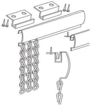
STRAIGHT TRACK
