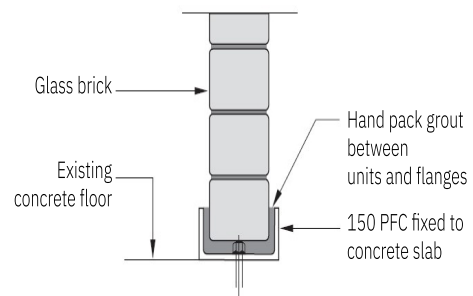
SECTIONAL ELEVATION
