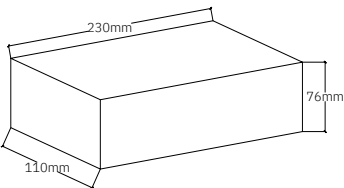
STANDARD BRICK
