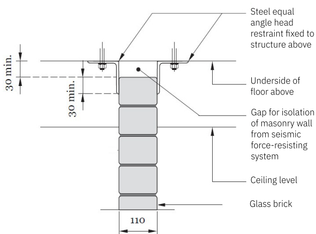
SECTIONAL ELEVATION
